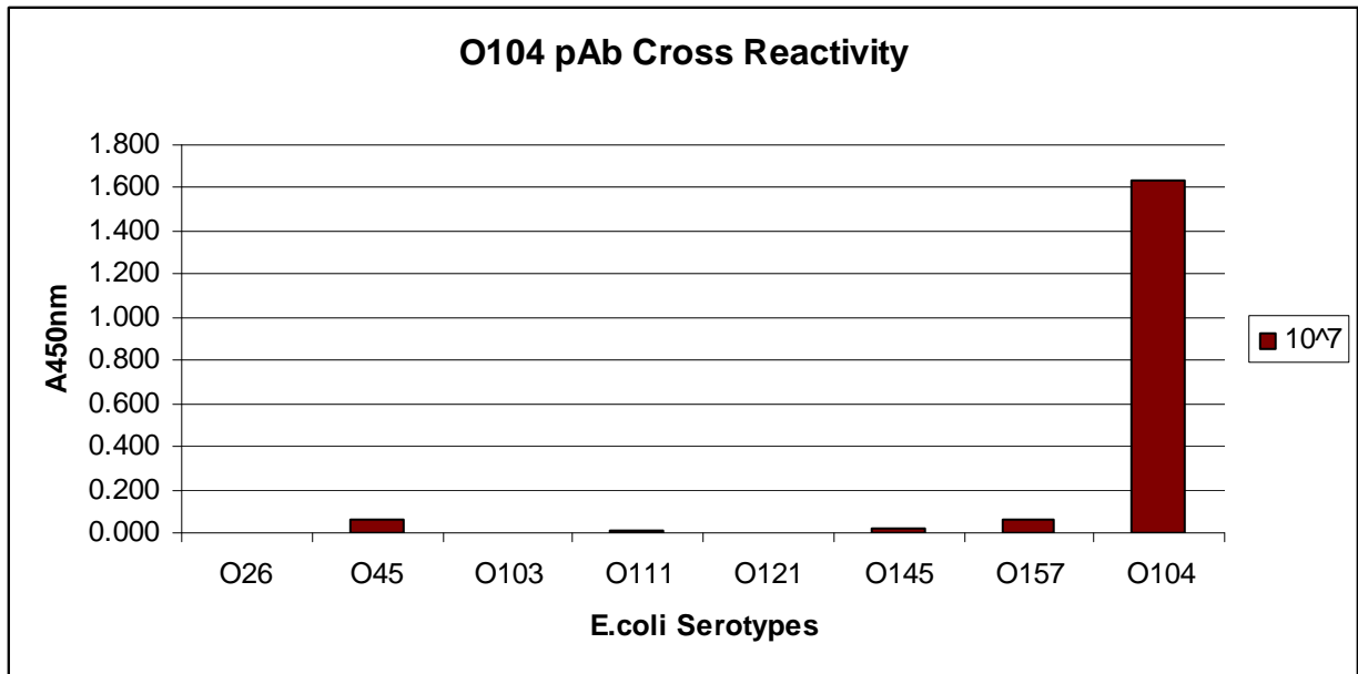
Cross Reactivity profile of E. coli O104 Polyclonal Antibody against 6 STEC and O157 with 10^7 cells coated onto microtiter plates using an indirect ELISA.
